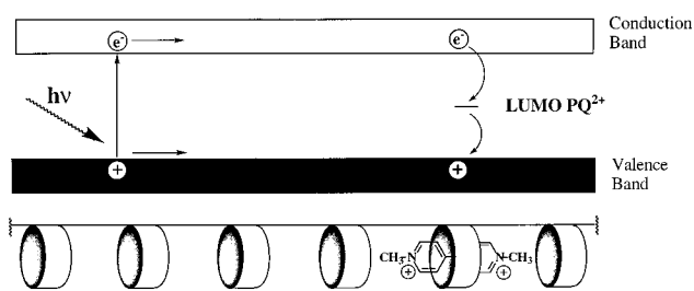
FIGURE 5. Schematic band diagram illustrating the mechanism by which the molecular wire receptor assembly can produce an enhancement in a fluorescence chemosensory response. The horizontal dimension represents the position along the conjugated polymer shown schematically at the bottom. Excitations are created by absorption of a photon ( h\nu ) and then migrate along the polymer backbone. Paraquat binding produces a trapping site whereby the excitation is effectively deactivated by electron-transfer quenching.
